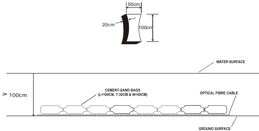
Fig.2. Sand-Cement Bags
